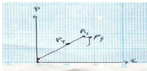
Gambar 9 kurva hasil uji tarik P ( kgf ) vs \epsilon (elongation) spesimen III.
