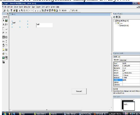
Gambar 3.1 Tampilan form
