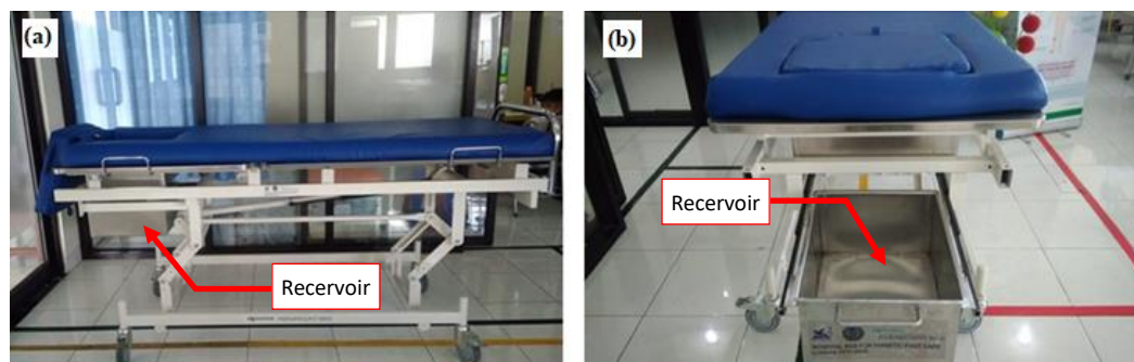
Figure 2. Prototype of HBDFUC developed by this research
