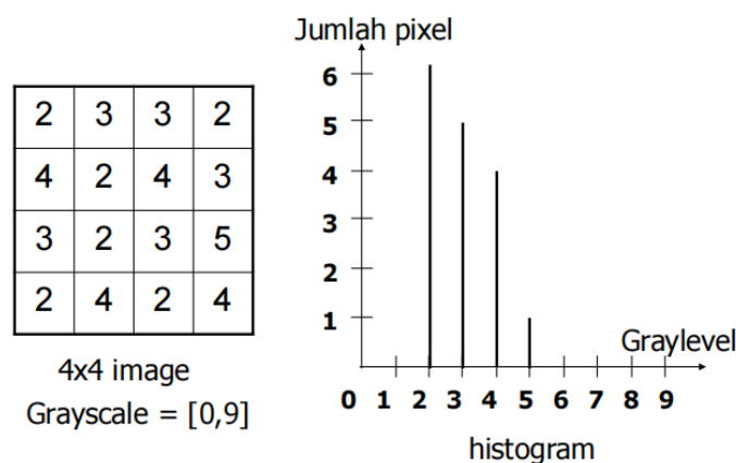
Gambar 3. Proses Perhitungan Histogram.
