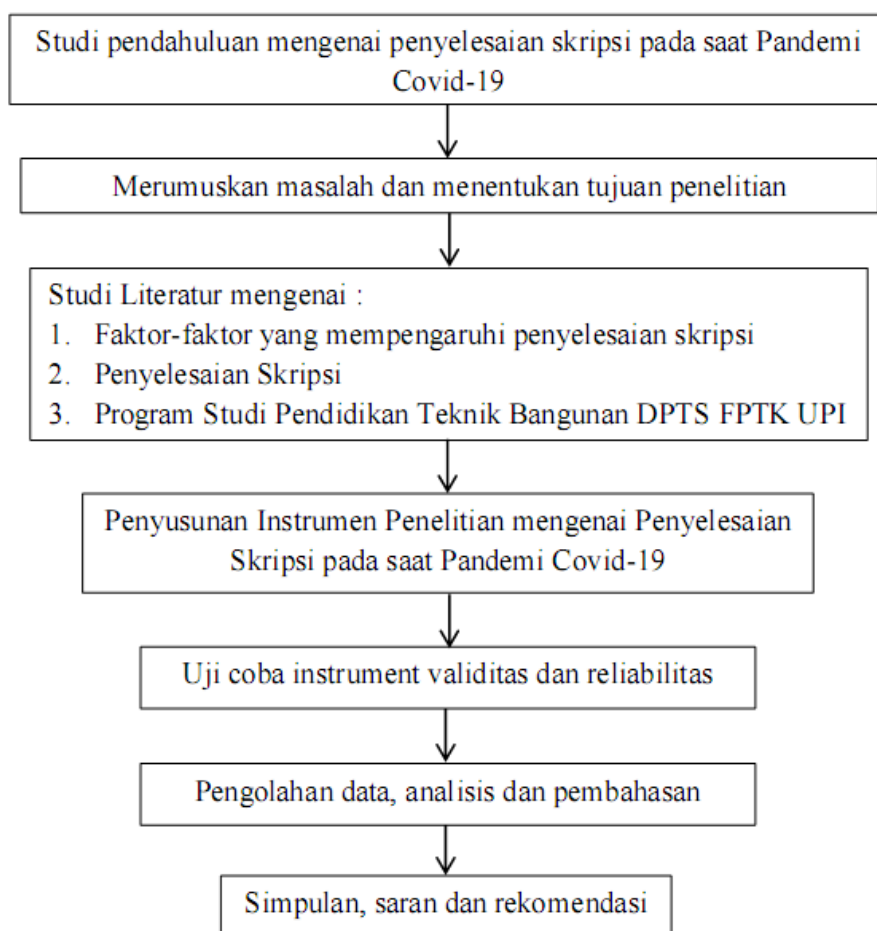
Gambar 1. Prosedur Penelitian
