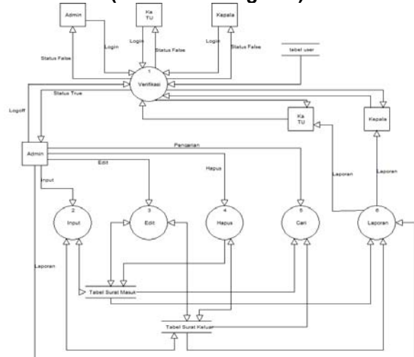
Gambar 3.2. DFD Level 0
