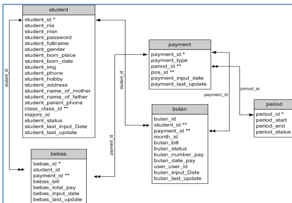
Gbr. 3 Logical Record Structure (LRS)
