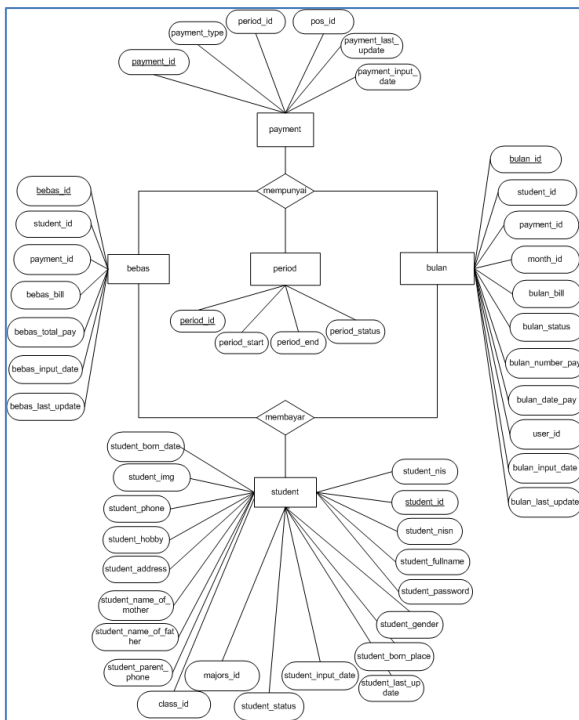
Gbr. 2 Entity Relationship Diagram (ERD)
