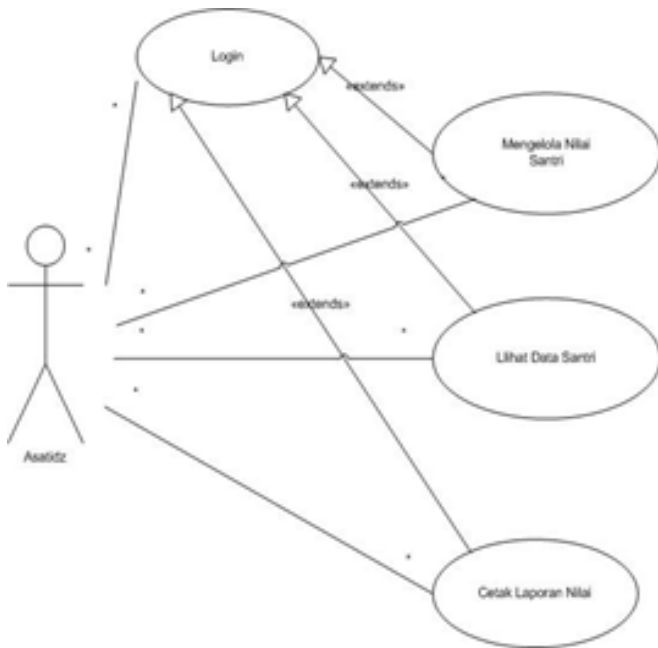
Gbr 2. Use Case Diagram Halaman Asatidz
