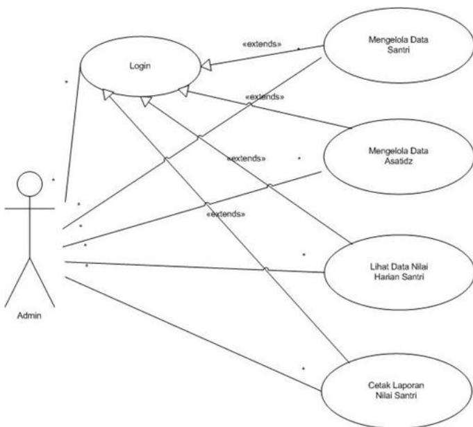
Gbr 3. Use Case Diagram Halaman Admin
