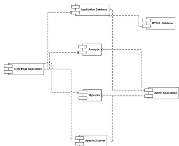
Gbr 9. Component Diagram Sistem Usulan
