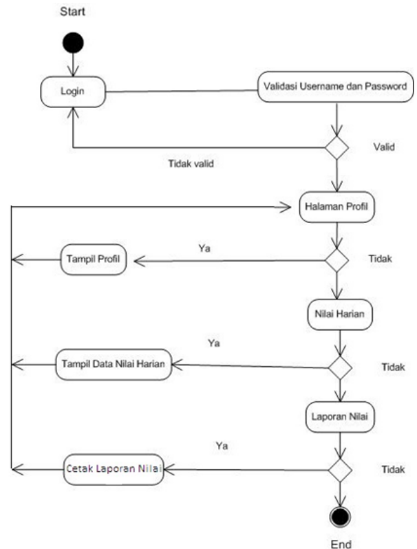
Gbr 4. Activity Diagram Halaman Santri Usulan
