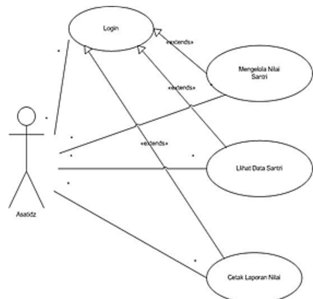
Gbr 1. Use Case Diagram Halaman Santri
