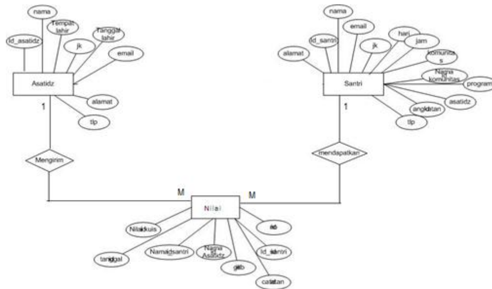
Gbr 10. Entity Relationship Diagram (ERD)
