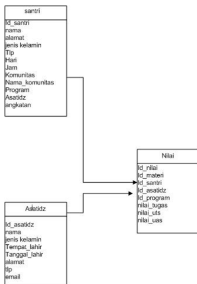
Gbr 7. LRS Sistem Usulan
