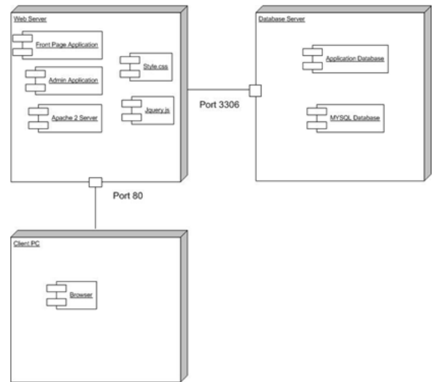
Gbr 8. Deployment Diagram Sistem Usulan
