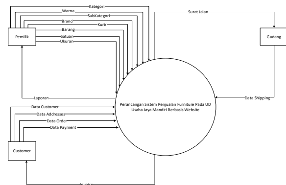
Gambar 1. Tampilan Context Diagram
