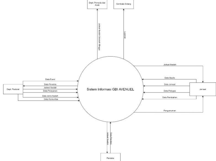
Gambar 2. Context Diagram
