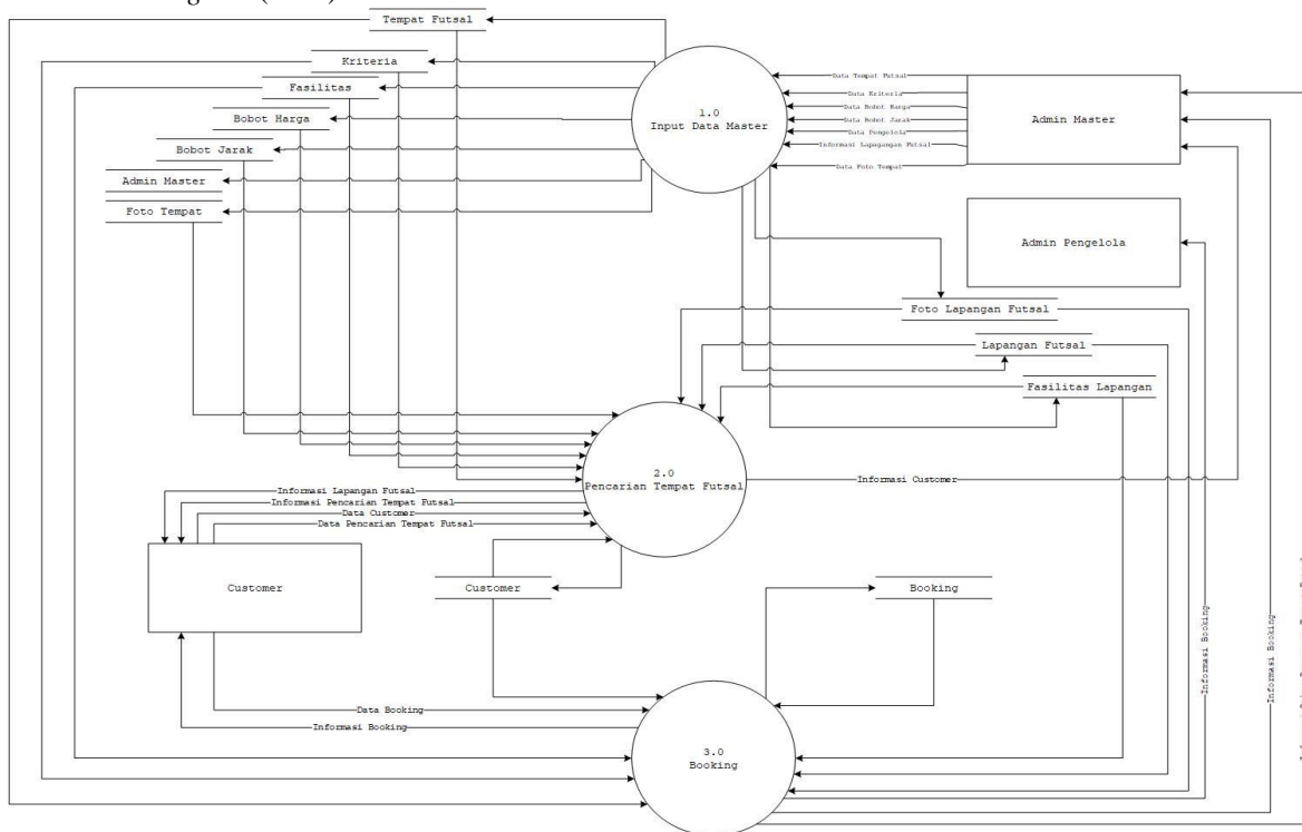
Gambar 2 Data Flow Diagram (DFD) level 0
