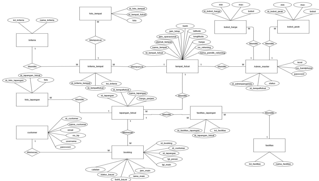
Gambar 3 Entity Relationship Diagram (ERD)
