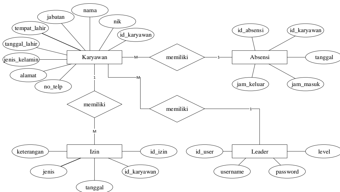
Gambar 2. ERD (Entity Relation Diagram)
