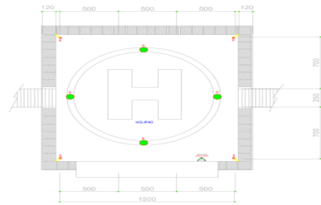
DENAH TATA LAMPU HELIPAD
