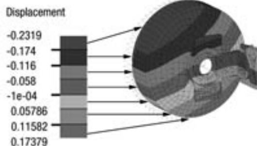
Finite element analysis displacement plot of antenna
