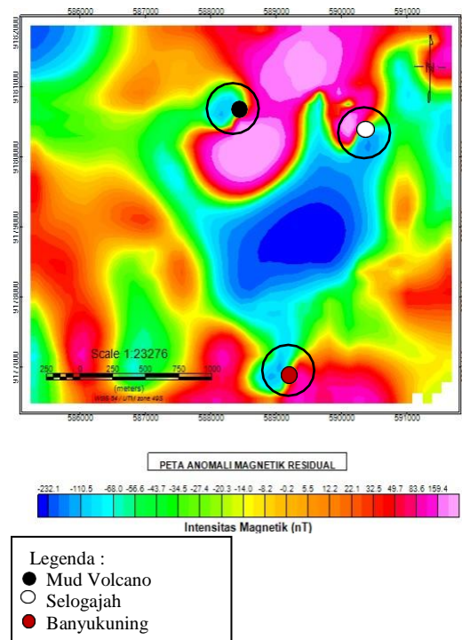
Fig 7. Residual Magnetic Anomaly Map in Gondang
