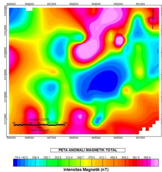
Fig 6. Regional Magnetic Anomaly Map in Gondang
