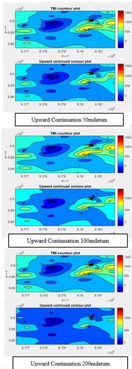
Fig 4. Comparison of datums in the Upward Continuation filter
