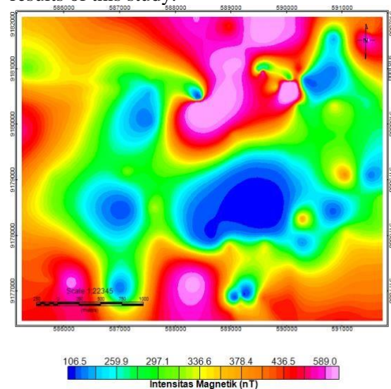
Fig 5. Total Magnetic Anomaly Map in Gondang
