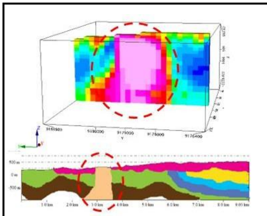
Fig 9. Comparison of geological section with the inversion model of the Jari mud volcano - Banyukuning
