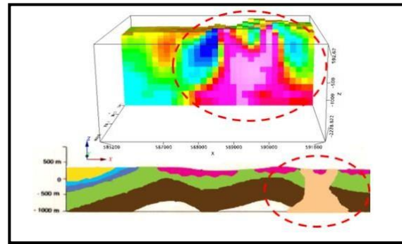
Fig 10. Comparison of geological incisions with the inversion model of the Selogajah Hot-Jari Mud Volcano
