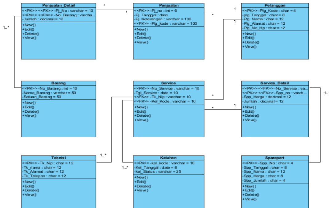
Gambar 4. Clas Diagram
