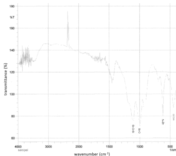
Figure 5. FTIR Spectra of synthesized \text{SiO}_2/\text{ZnO} nanocomposites
