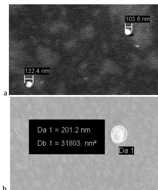
Figure 4. SEM images of \text{SiO}_2/\text{ZnO} composites (a) size range 103–132 nm (b) (size range 201.2 nm)
