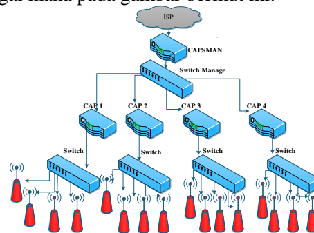
Gambar 3. Blok Diagram WMN
