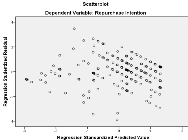
Fig. 3 Heteroscedasticity Test
