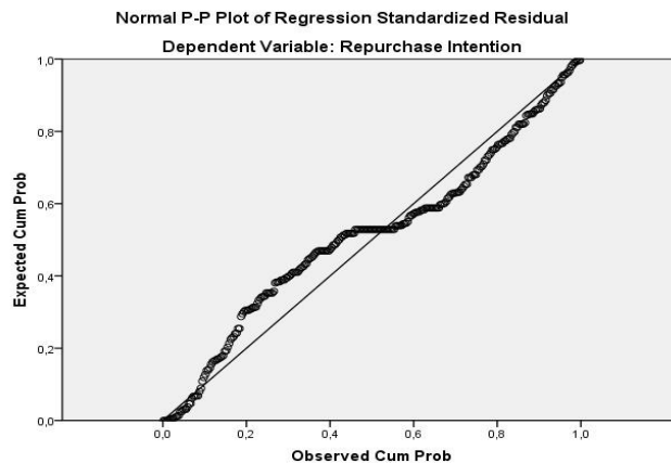
Fig. 2 Normality Test Results
