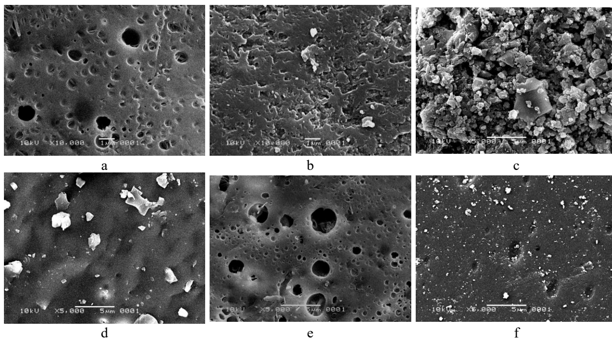
Figure 2. SEM images of (a) EOA-Cr-EGDMA, (b) EOA-EGDMA, (c) Eug-Cd-DVB %, (d) Eug-DVB 10%, (e) Poly-Cr-DVB, (f) Poly-DVB
