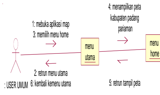
Gambar 3. Collaboration Diagram
