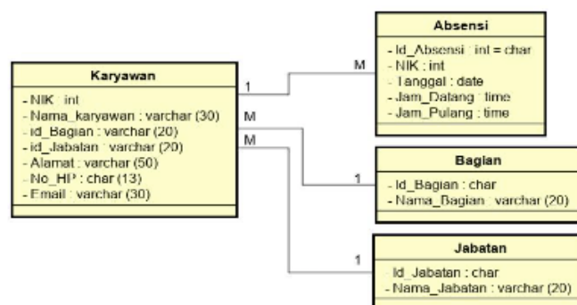
Gambar 3. Class Diagram
