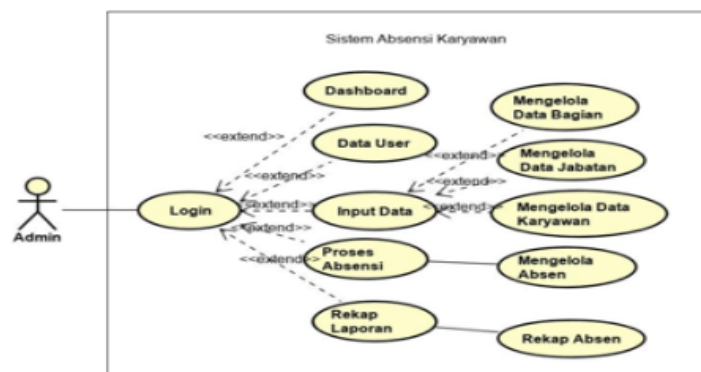
Gambar 2. Usecase Diagram
