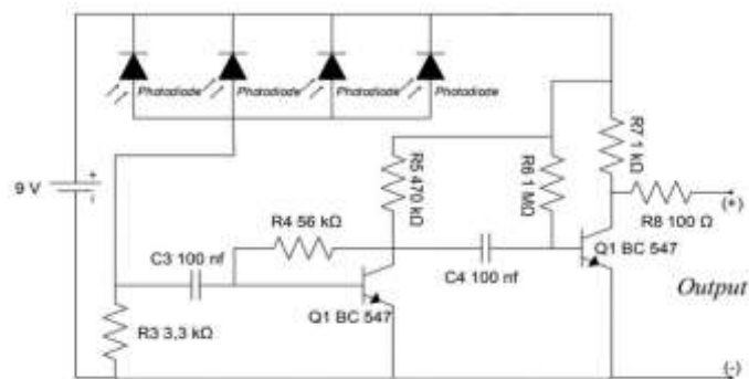
■ Gambar 8. Rangkaian VLC Receiver
