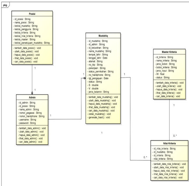
Gbr. 7. Class diagram
