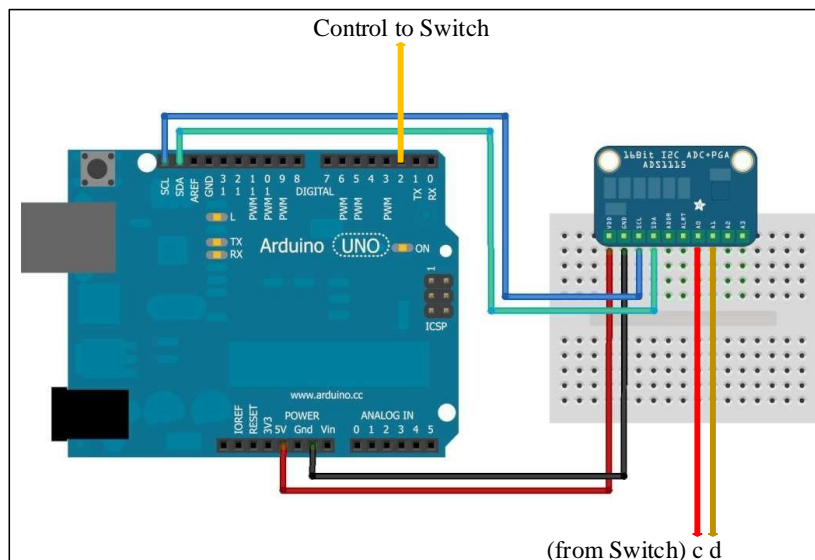
Figure 5. Arduino Uno and ADS1115 assembly (modified from [11] and [13])
