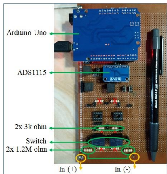
Figure 6. Voltmeter prototype
