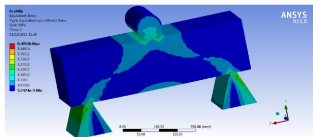
Figure 14. Typical (von - mises) Stress for a Modelled Beam
