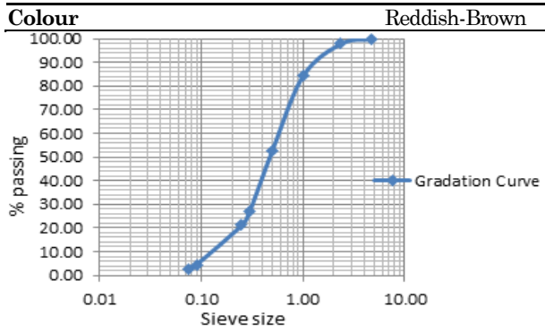
Figure 10. Particle Size Distribution Curve of the Laterite Used
