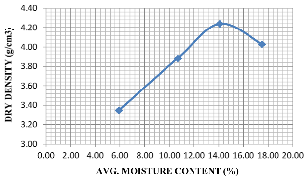
Figure 11. Dry Density Against Average Moisture Content
