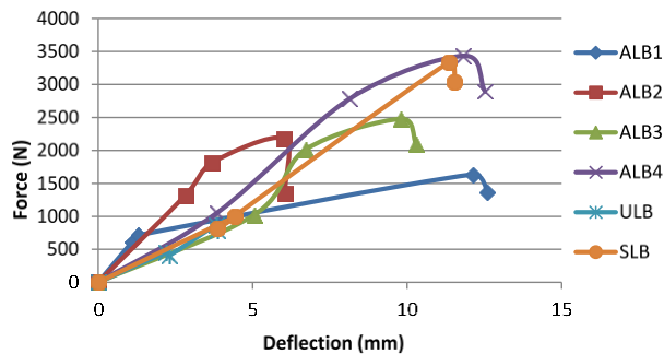
Figure 13. Load-deflection Curve for the Unreinforced, Steel, and Apa Reinforced Soil Beams
