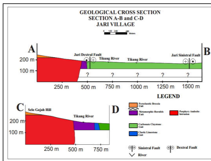
Fig. 4. Geological cross section of Jari Village, Gondang Sub-District, Bojonegoro District
