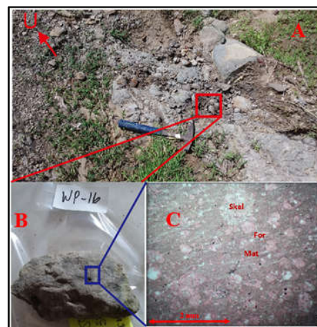
Fig. 6. (A) The outcrop of marls at STA 28 (B) Handspecimen of marls (C) Petrographic appearance of marls
