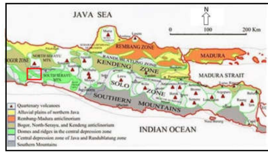
Fig. 1. Physiography of Eastern part of Java (Van Bemmelen, 1949)
