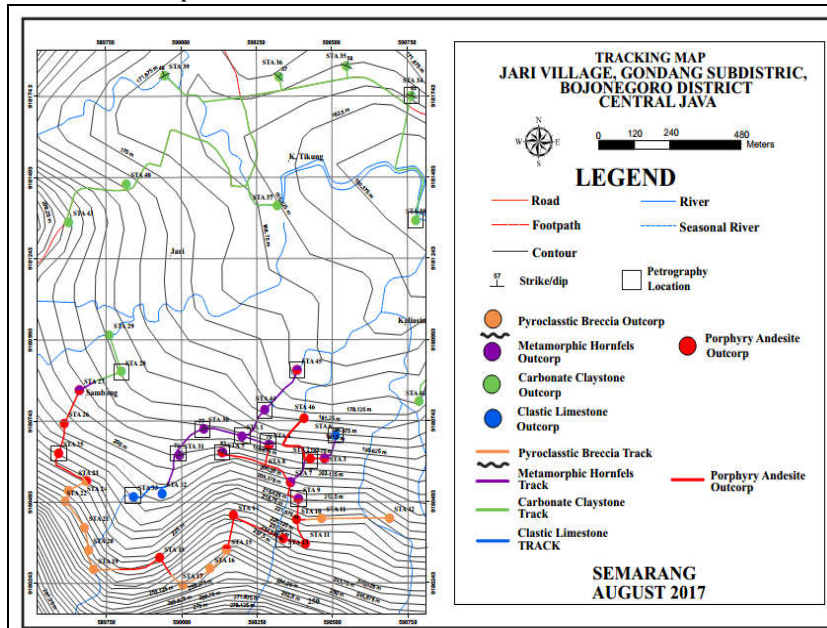
Fig. 10. Tracking map of Selo Gajah Hill, Jari Village, Gondang Sub district, Bojonegoro District
