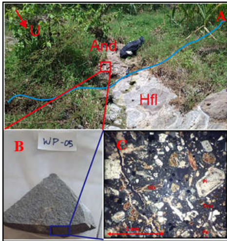
Fig. 7. (A) The contact of porphyritic andesite intrusion (And) and hornfels (Hfi) at STA 9 (B) Handspecimen of porphyritic andesite (C) Petrographic appearance of porphyritic andesite
