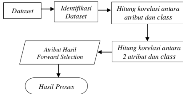
Gambar 2. Kinerja model Forward Selection
