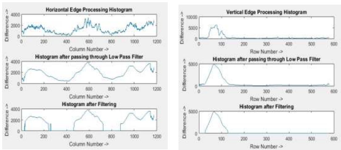
Gambar 3. Histogram Approach Horizontal Projection dan Vertical Projection
