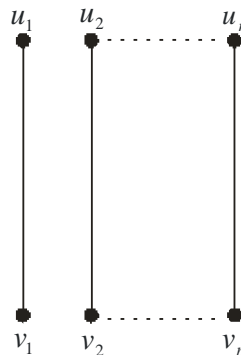
Figure 1. The ladder rung graph
