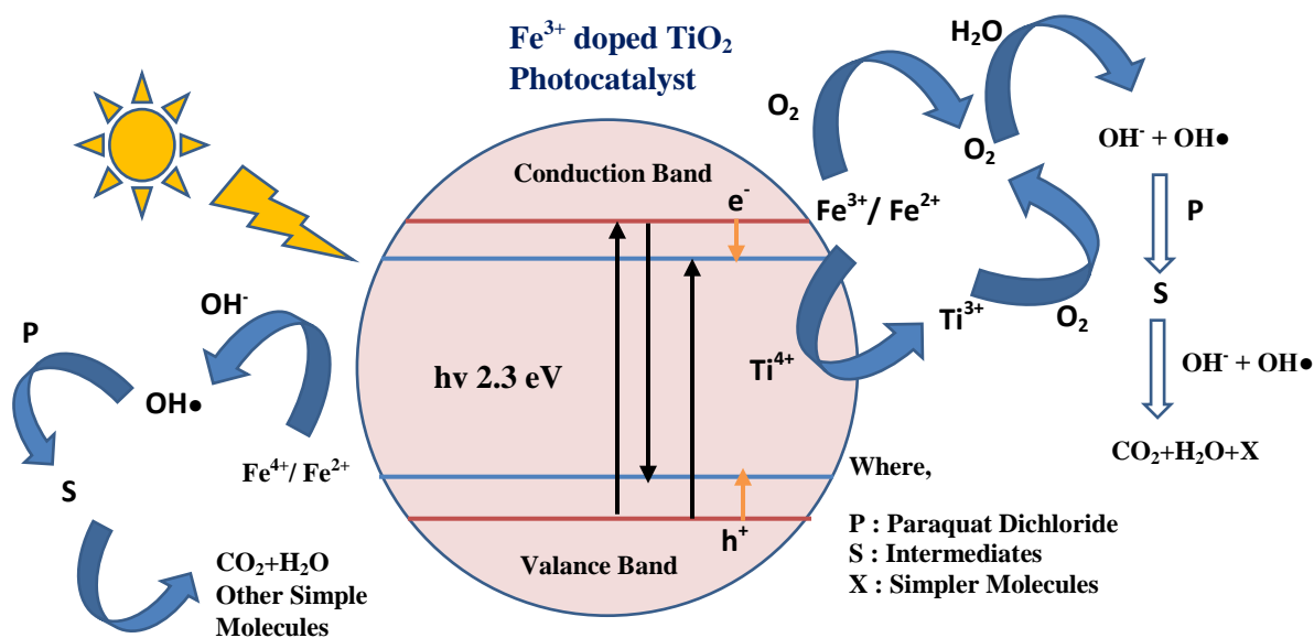
Figure 7. Schematic illustration of the energy diagram for a Fe-TiO 2 system
