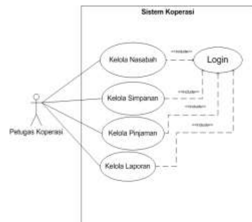
Gambar III-1. Diagram Use Case
