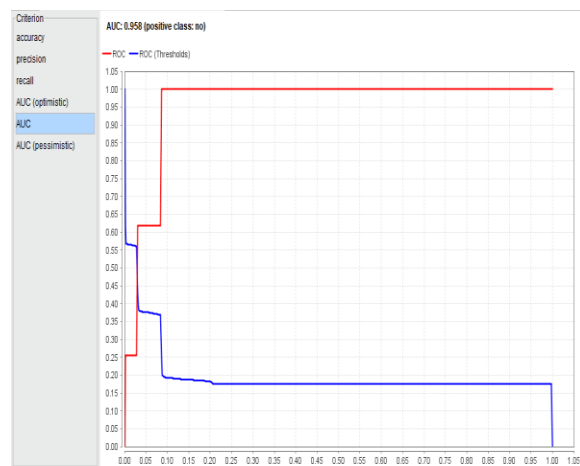
Figure 6. K-NN ROC curve
