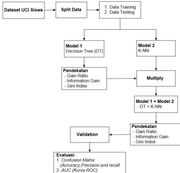
Source : (Saputri et al., 2020) Figure 1 Research Methodology
