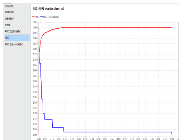
Figure 5. ROC Decision Tree Curve with Information Gain
