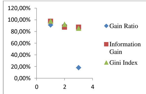
Source : (Saputri et al., 2020) Figure 2 Scatter Diagram of Decision Tree Results Tree
