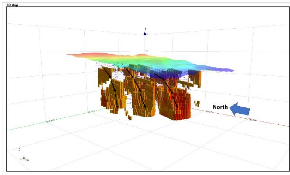
Fig. 13. Side view of 3D model of resistivity interpreted as aquifer.
