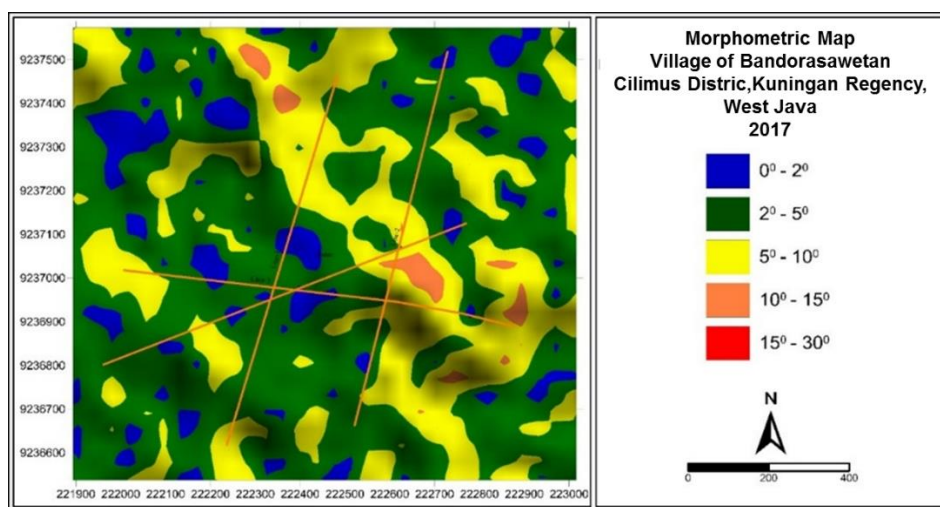
Fig. 3. Morphometry of research area.
