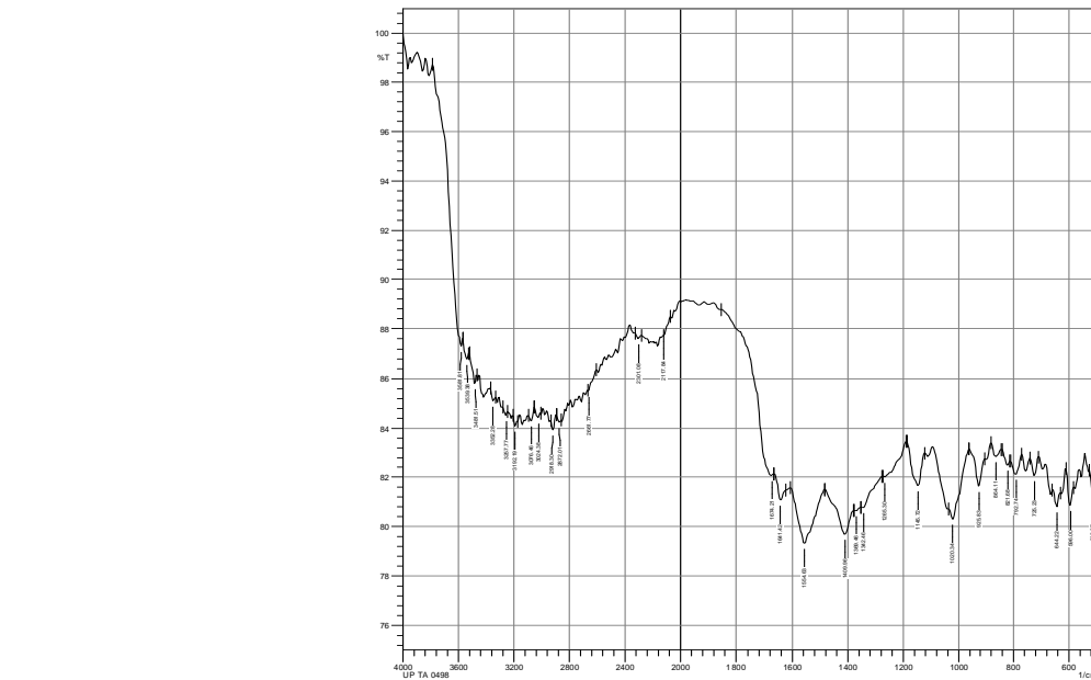
Gambar 4. Spektra FTIR Standar Beta D-glukan dari Barley (Sigma) (a), beta glukun jamur tiram larut air (b), beta glukun jamur tiram larut alkali (c)
