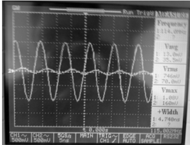
Gambar Gelombang Input dan Band High Pass Filter
