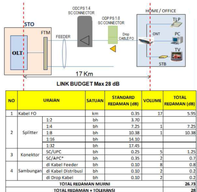
Figure 6: Link Budget Linking Standards [1]
