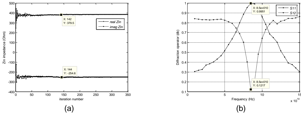
Figure 5. (a) Imaginary and Real Part of Z_{in} as Function of Iteration Number (b) Diffraction Operator as Function of Frequency
