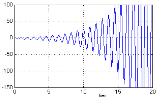
Fig. 4 Response of an un-compensated system.
