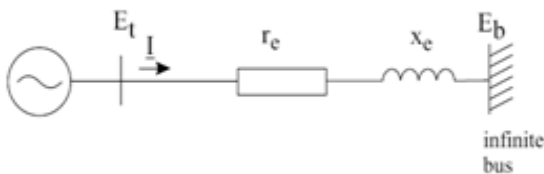
Fig.1 One machine to infinite bus.
