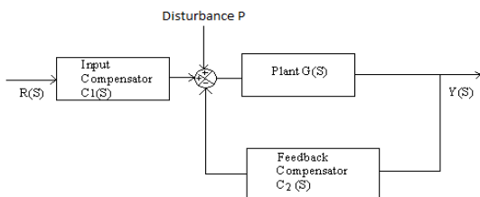
Fig. 2. Two Parameter controller configuration.
