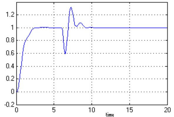
Fig. 6 Response for a disturbance, with internal model principle design
