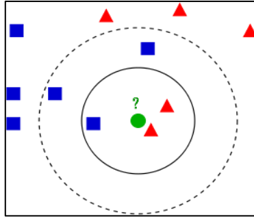
Figure 6. k-NN classification
