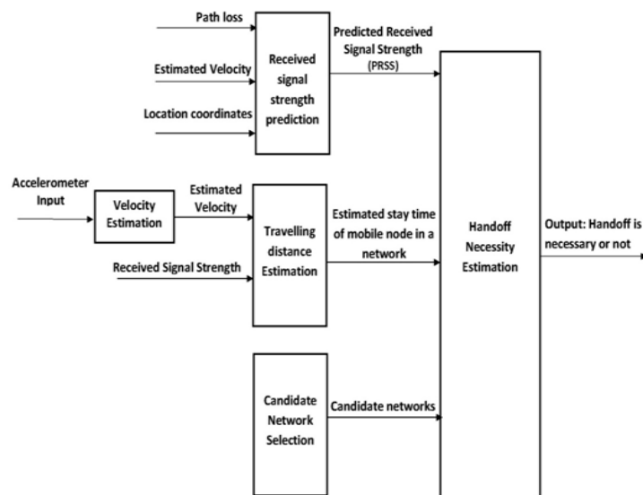
Figure 3. Handoff necessity estimation module (HNEM)
