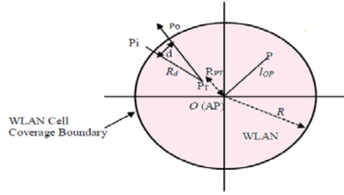
Figure 5. Travelling distance estimation with respect to radius at point P_T
