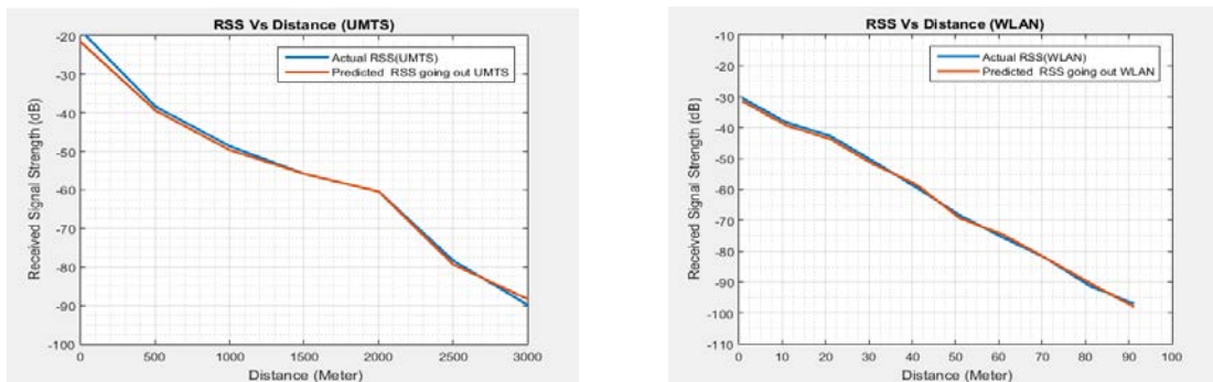
Figure 7(a): PRSS of mn moving out from UMTS
