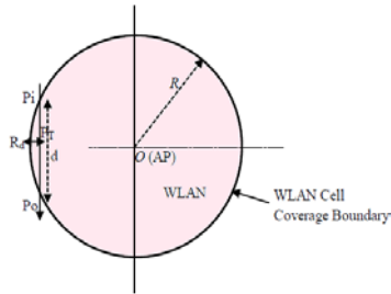
Figure 2 (a): Travelling distance w.r.t radius (Rd) in overlapping structure
