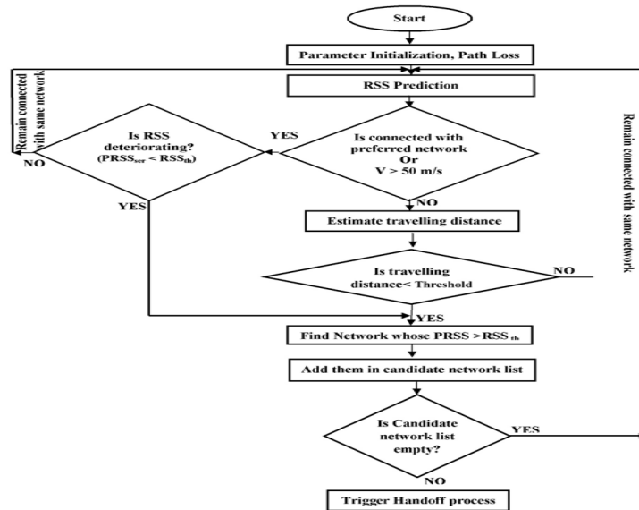
Figure 6: Flowchart of handoff necessity estimation algorithm.
