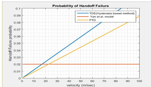
Figure 10: Handoff failure probability vs. velocity
