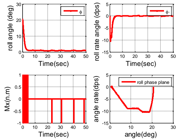
Figure 7a. Roll angle operation of fuzzy on-off controller (T-S model)
