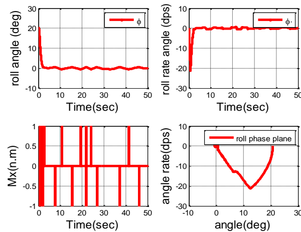
Figure 7b. Roll angle operation of optimized fuzzy on-off controller (T-S model)
