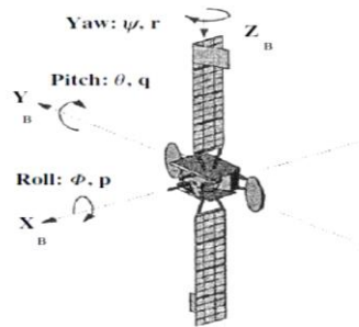
Figure 1. Satellite reference and body coordinates [17]
