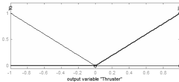
Figure 4. Output Membership functions
