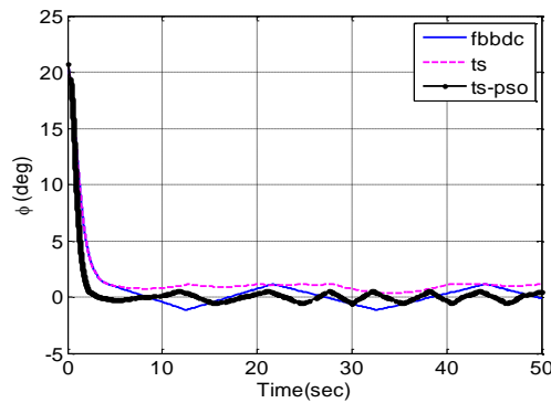
Figure 8. roll angle comparison of controllers
