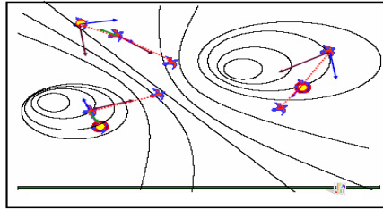
Figure 5. General structure of particle swarm algorithm
