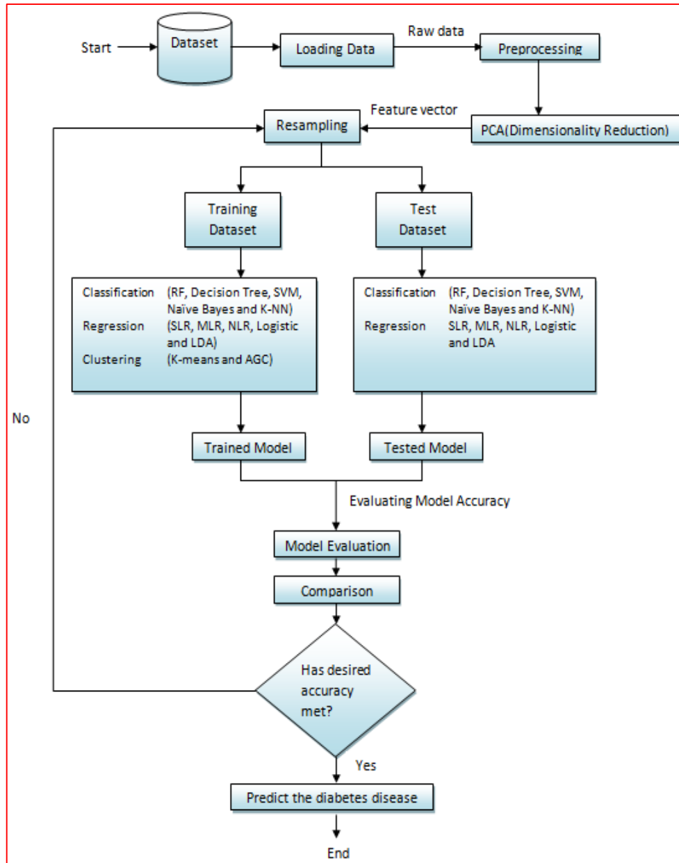
Figure 1. Proposed system for diabetes prediction system
