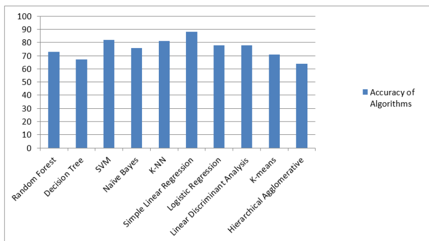
Figure 2. Comparison of accuracy of various algorithms
