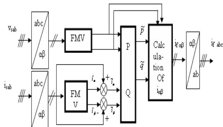
Figure 3. The Method of Instantaneous Active and Reactive Power
