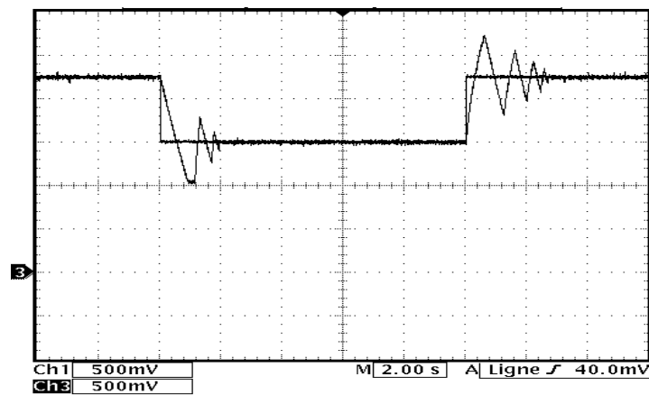
Figure 13. Experimental APF results with PI: DC voltage V_{dc} (V) and DC reference voltage V_{dc}^* (V), Ch1 and Ch3 scale: 100 V/div, Time scale: 2s/div.
