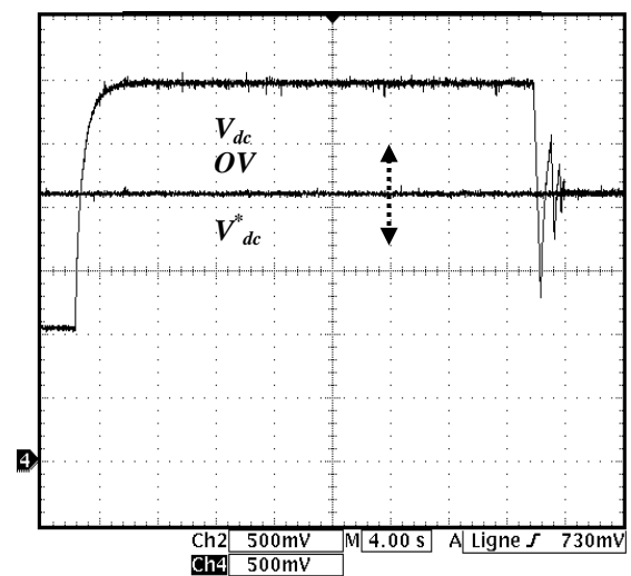
Figure 10. Experimental APF results with PI: DC voltage V_{dc} (V) and DC reference voltage V_{dc}^* (V), Ch2 and Ch4 scale: 100 V/div. Time scale: 4 s/div.
