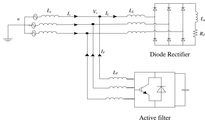
Figure 1. Power System Configuration.
