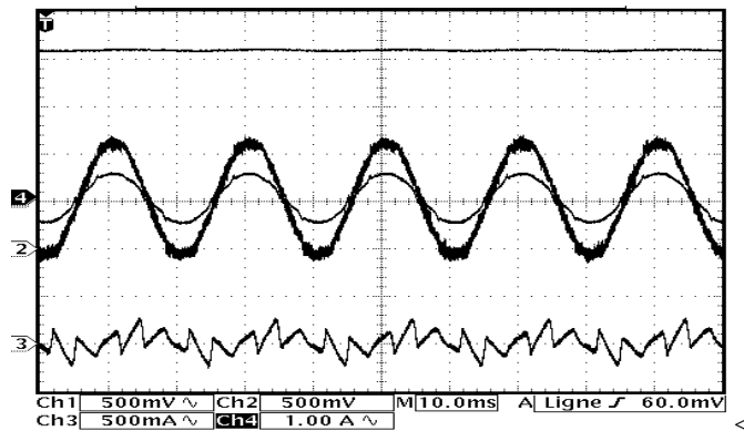
Figure 6. Experimental results: filter current i_f (A), source current i_s (A), source voltage V_s (V) and DC voltage V_{dc} (V). Ch3 and Ch4 scale: 5 A/div; Ch2 scale: 100 V/div; Ch1 scale: 80 V/div; Time scale: 10 ms/div.
