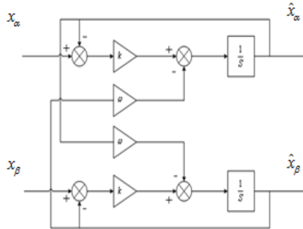
Figure 4. Self Tuning Filter
