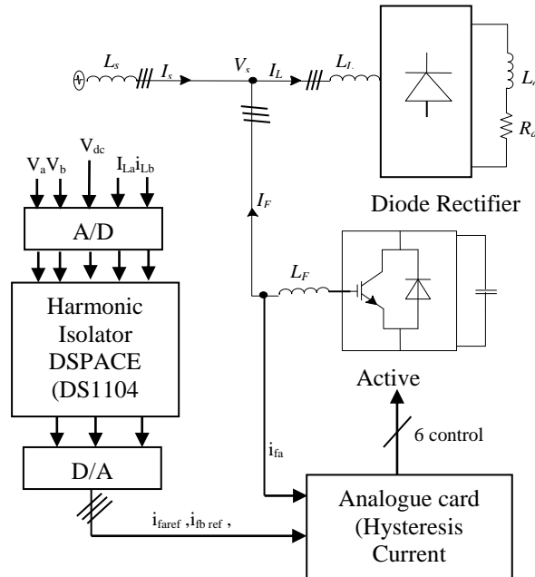
Figure 2. Experimental System
