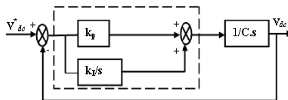
Figure 5. Scheme with PI controller of the DC-link voltage.
