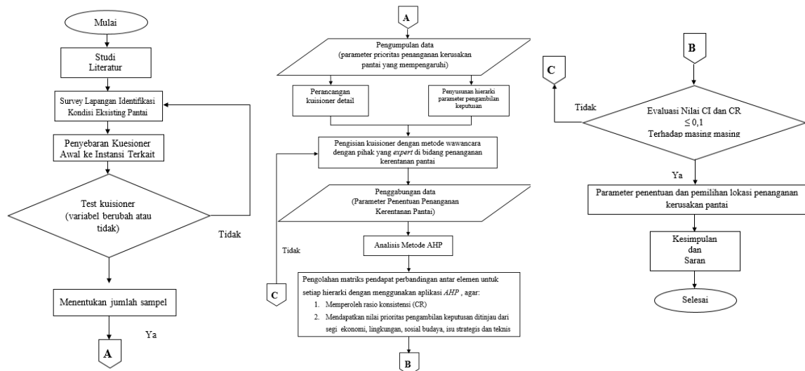
Gambar 3. Flowchart penelitian
