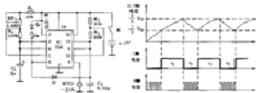
Gambar 9. Animasi CircuitMaker
