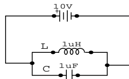
Gambar 12. Rangkaian L-C (CircuitMaker 2000 software)
