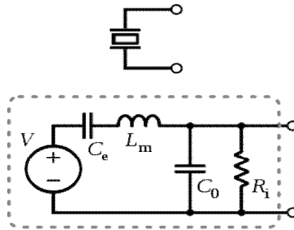
Gambar 2. Piezoelectric Transducer
