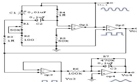
Gambar 19. Osilator Fungsi
