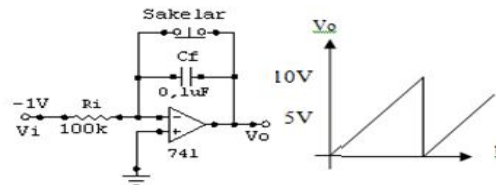
Gambar 18. Osilator Gigi Gergaji
