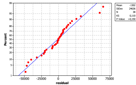
Gambar 3. Plot Normalitas Residual
