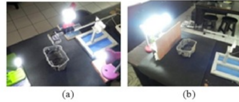
Figure 8. Capturing; (a) Direct; (b) Diffuse
