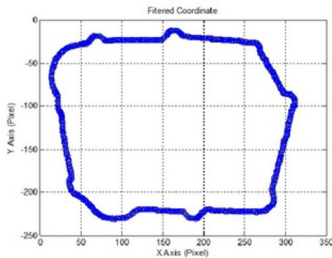
Figure 14. Filtered coordinate
