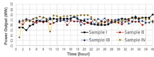
Figure 9 Power Output
