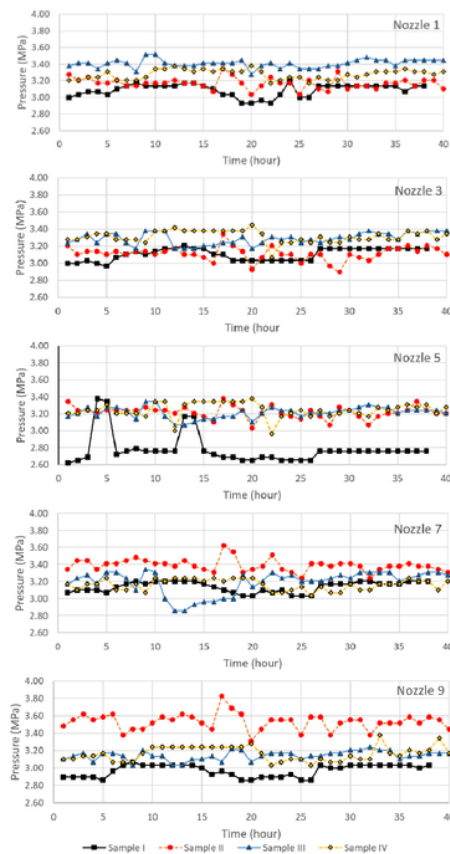
Figure 13 Nozzle Pressure Profile
