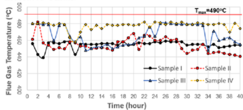
Figure 16 Profile of Flue Gas Temperature
