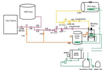
Figure 6 Sub-facilities of Blending Facility
