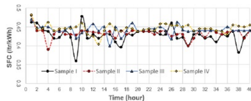
Figure 10 SFC Profile
