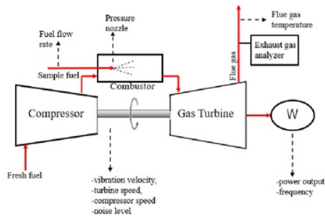
Figure 3 Flowchart of the Experiment
