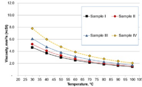
Figure 7 Effect of an Increase in Temperature on a Sample Viscosity
