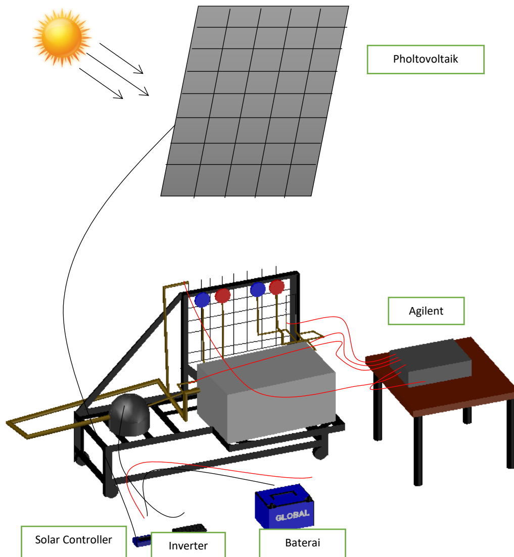
Gambar 3.2 Set-Up Experimental
